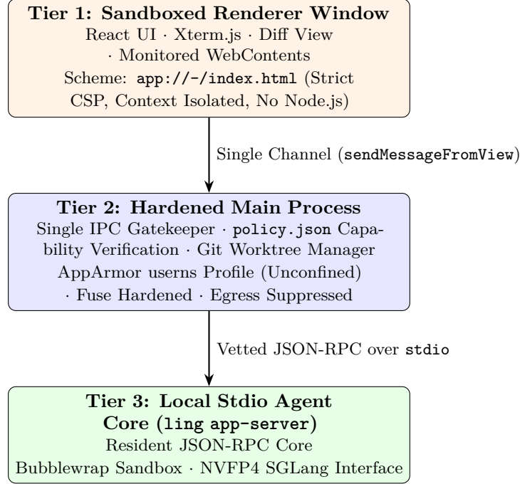
Figure 1: Three-tier architecture of Mightling Desktop: Sandboxed Renderer, Policy-Vetted Main Process, and Stdio Agent Core.
